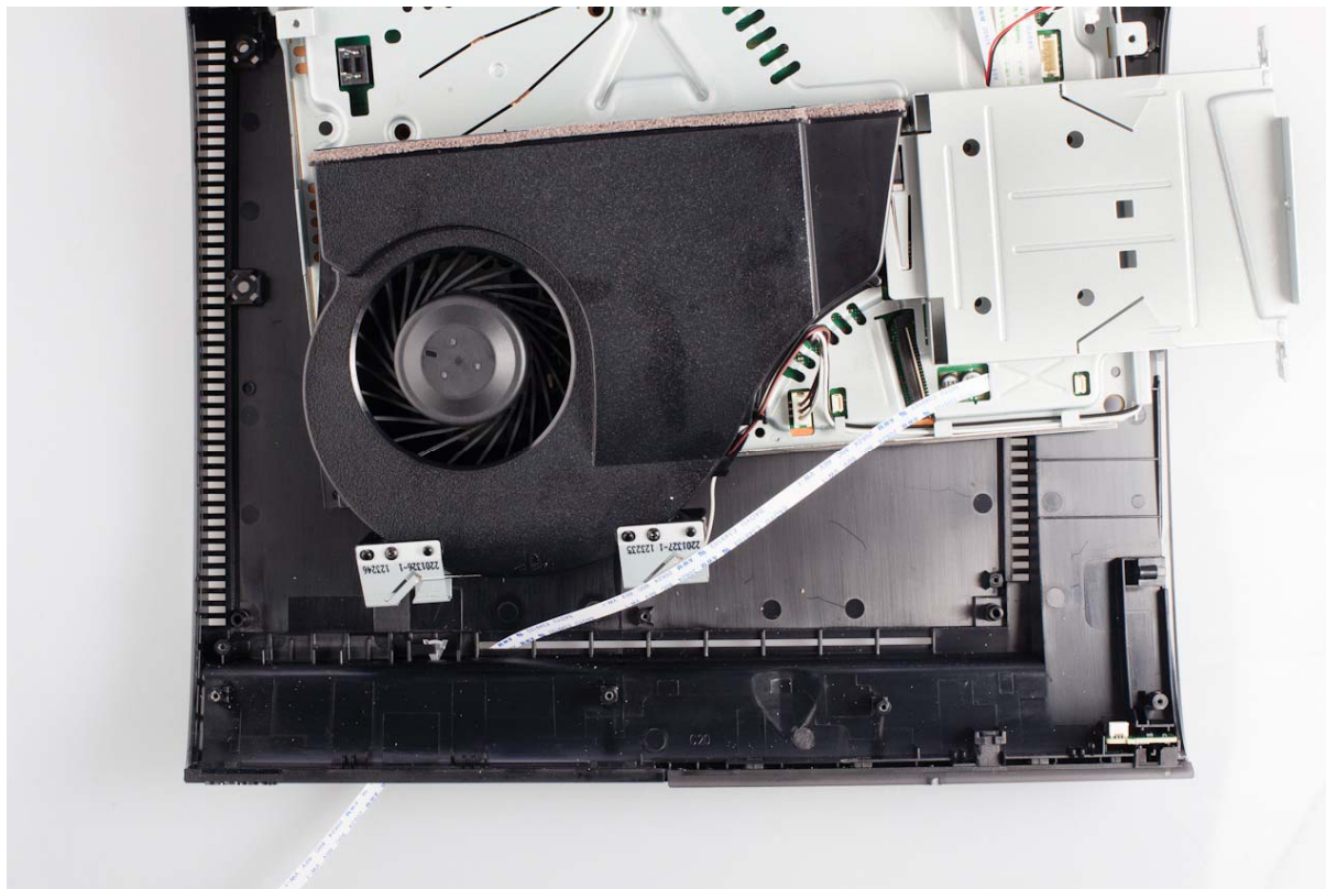
Illustration 10: Routage de la nappe USB
