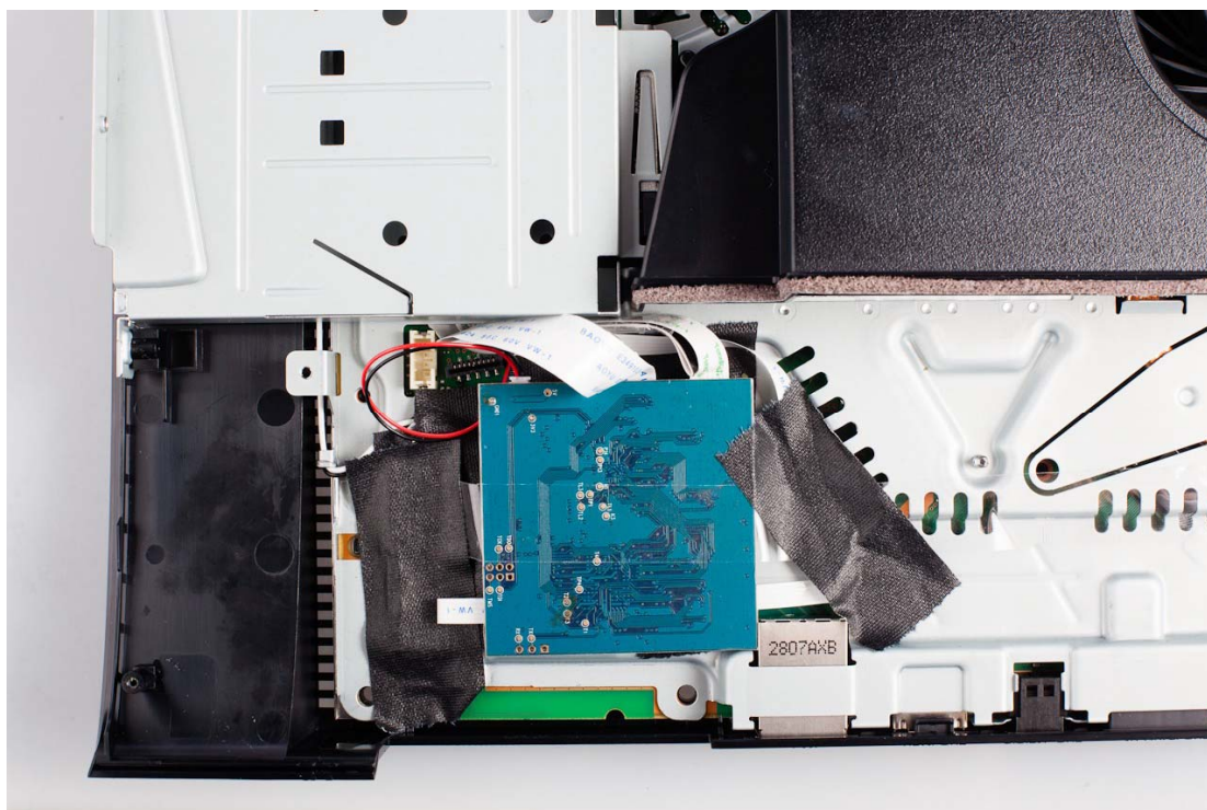
Illustration 13: Installation du 3K3Y PCB
