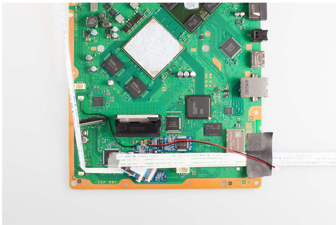
Illustration 8: Pliage des nappes souples
